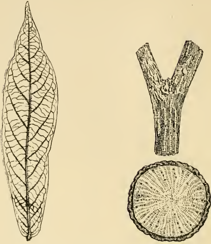
ANTIDOTE NO. 1.—SKETCH OF LEAF AND STEM.
